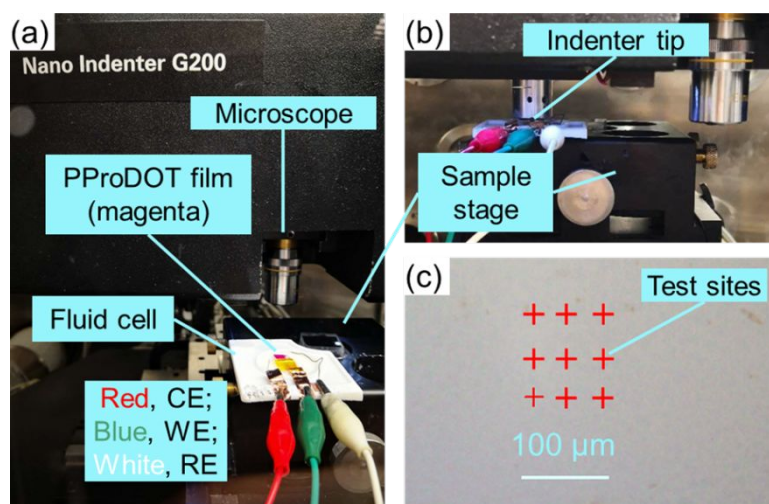
Figure S1. The experimental setup of the in-situ measurement of mechanical strain in PProDOT. (a) Fluid cell with the PProDOT film, Ag/AgCl reference electrode, and Pt counter electrode mounted on the sample stage. The copper wire connecting the ITO substrate is covered with electrochemically inert epoxy. (b) Indenter tip on the sample. (c) nine indentation sites under the microscope.
