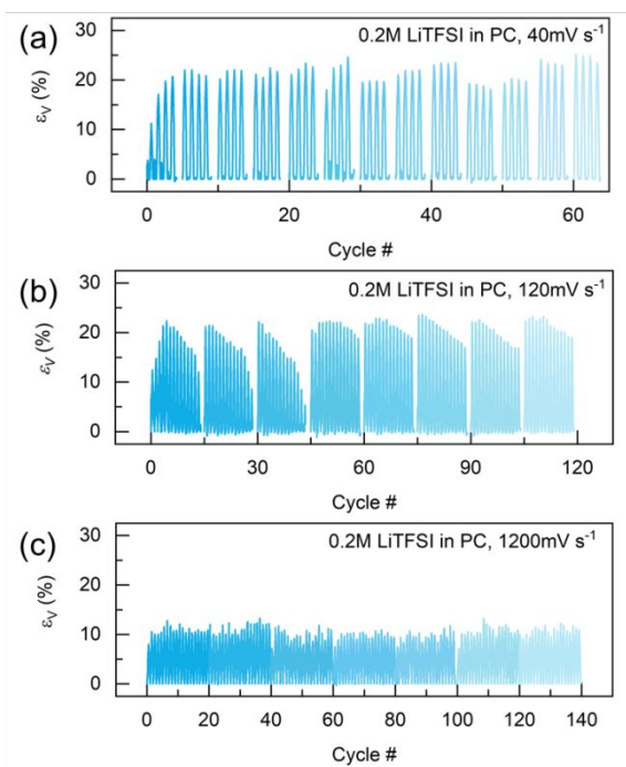
Figure S4. Breathing strain of the PProDOT film for different scan rates. (a) 40 \text{ mV s}^{-1} , (b) 120 \text{ mV s}^{-1} , and (c) 1200 \text{ mV s}^{-1} .
